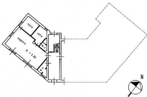
PIANO TERRENO
